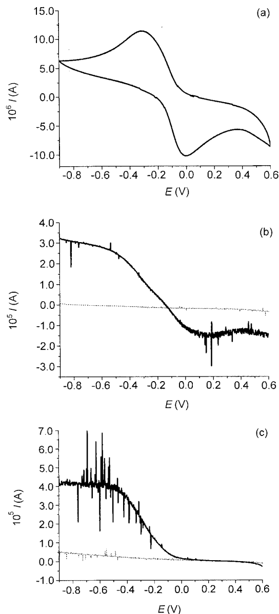
Figure 4. Cyclic voltammogram for 1 at a scan rate of 0.02 V s −1 (a); normal pulse voltammogram (NPV) with anodic scan of 1 (b); NPV with cathodic scan of 1 (c)
