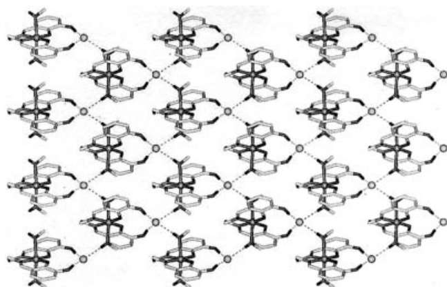
Figure 3. Perspective view of the 2D network formed, which shows the chloride's role as supramolecular glue in the assembly of the manganese(III) complexes
