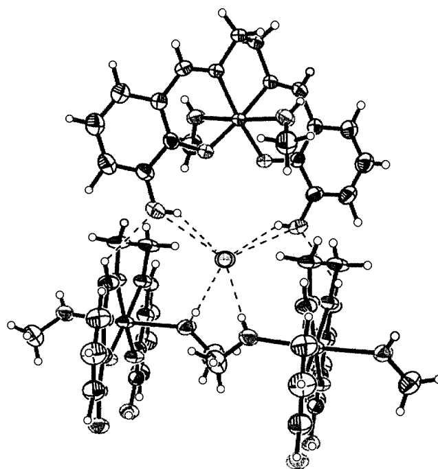
Figure 2. Part of the unit cell of 1 , exhibiting the net of interactions between three neighbouring cationic complexes; the chloride anion is tetra-coordinated to four hydroxy groups through hydrogen bonding
