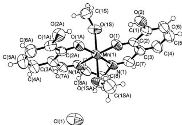
Figure 1. ORTEP plot of 1 ; atoms showing the atomic numbering scheme are represented by their 50 % probability ellipsoids; symmetry operation to generate equivalent atoms: A = x + 2, y, -z + 1/2
